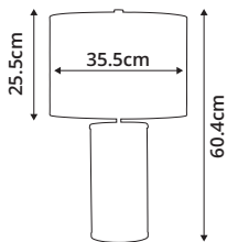
QN-RENO-SMOKE-PN 1 Lt Table Lamp Materials: Steel, Optical Glass, Faux Silk Finish: Polished Nickel Shade: Whale grey faux silk with silver metallic inner Max W: 1 x 60W E27
