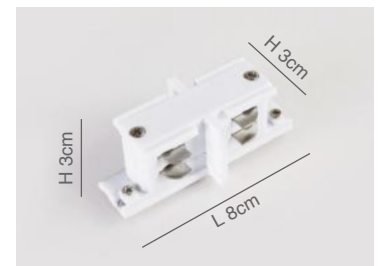
77-9112-3 Trio Straight Connector White
