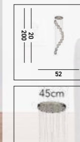
97291-12SM CYCLONE 12Lt Multi-Drop Pendant Chrome Metal & Smoked Glass
